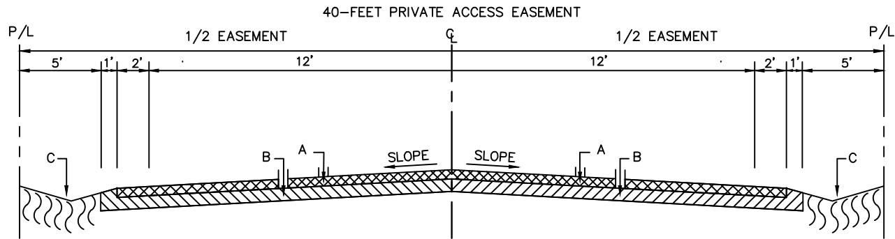
TYPICAL SECTION
