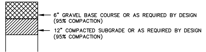
ROADWAY SECTION
